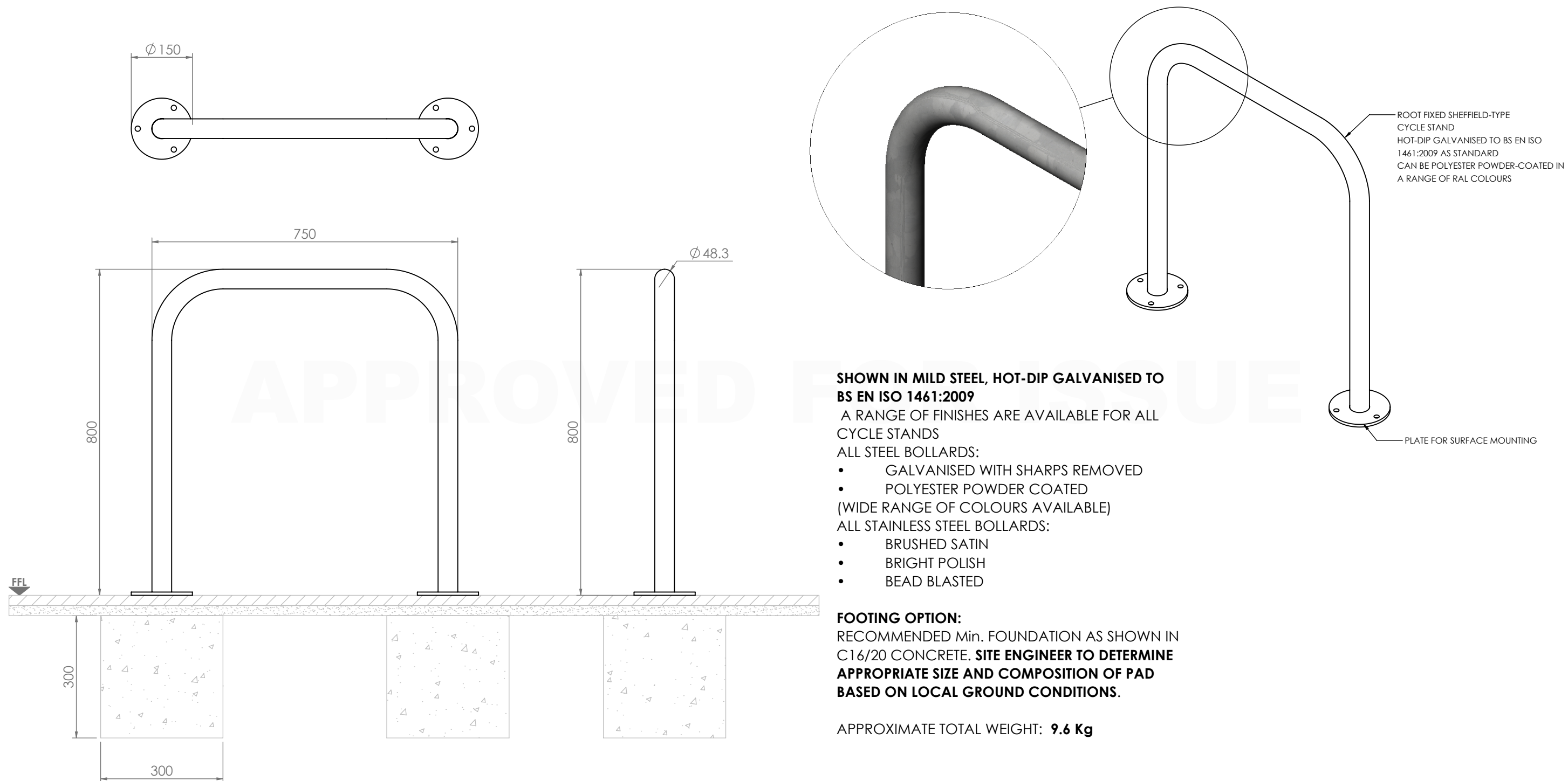
SHEFFIELD CYCLE STAND SM CIRCULAR PLATE GENERAL ARRANGEMENT
